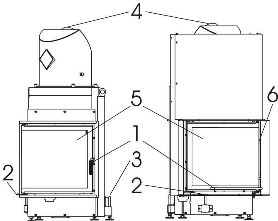
Im. 1: Eck-Kamin with side-opening / lifting door (shown with steel hood, as an example)
